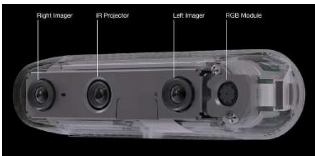
Figura 16: Intel RealSense D435 .
